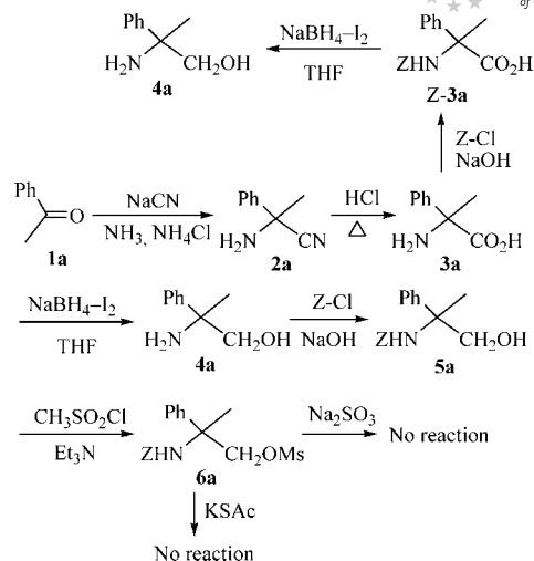
Scheme 1. Attempt to synthesize N -Z-protected 2,2-disubstituted taurines.
