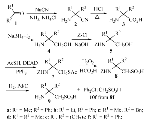
Scheme 2. General route for the synthesis of N -Z-protected and free 2,2-disubstituted taurines.
